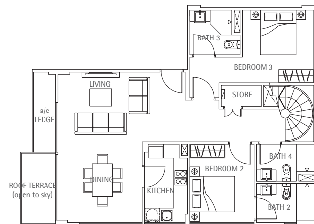
Type CP2 #07-15 180sqm / 1,938sq ft
