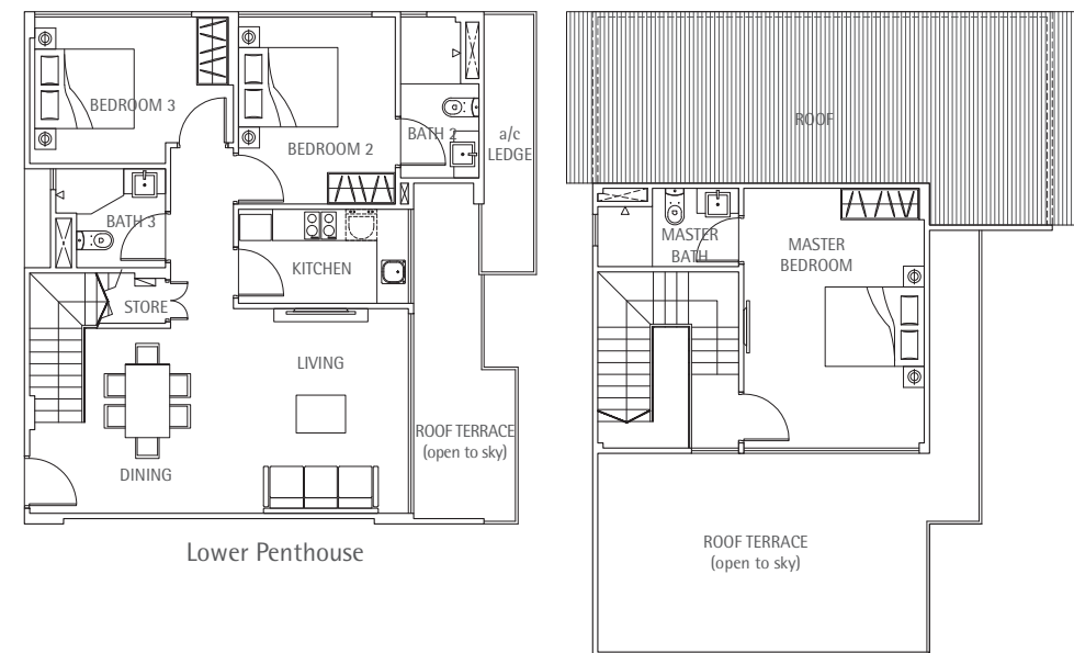
Lower Penthouse Type CP #08-11 153sqm / 1,647sq ft
